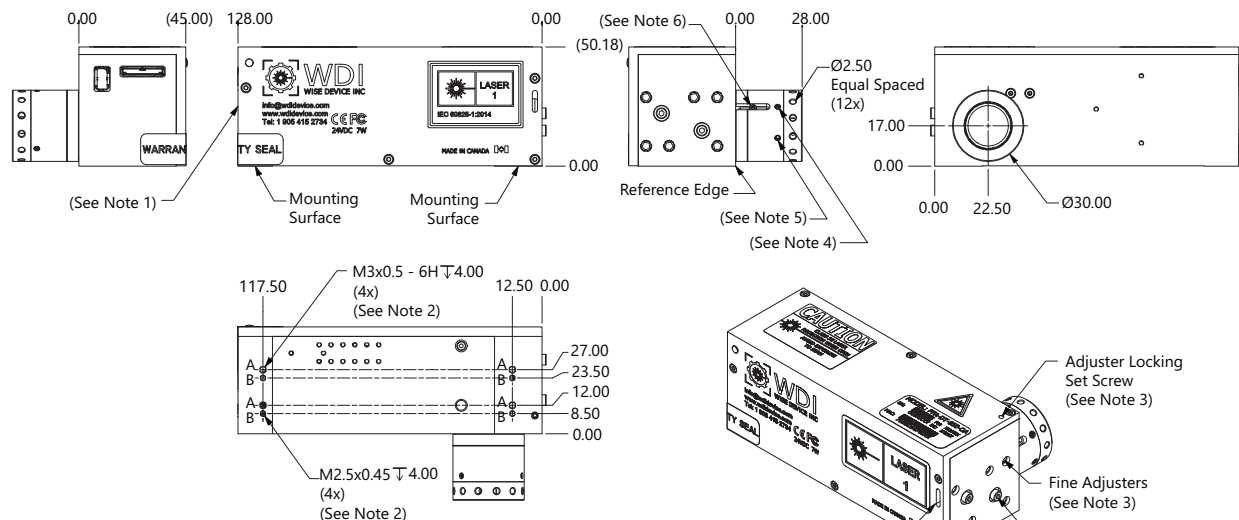
Figure 4 PFA-DT Sensor Dimensions
